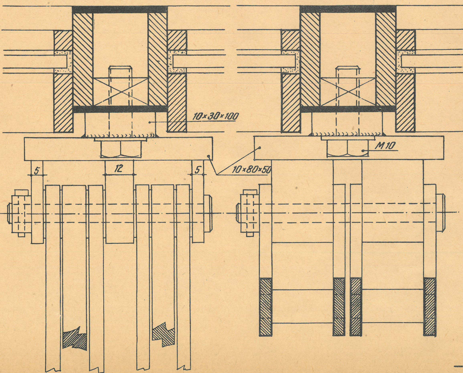
PLAN NOD A
